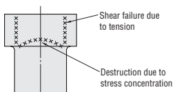
[Fig. 4] Punch head destruction
