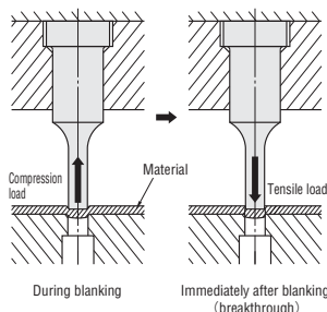
[Fig. 2] Conditions of tensile force generation
