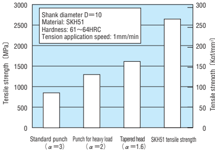
[Fig. 6] Punch head tensile strengths for different punches (D=10, SKH51) \alpha : Stress concentration coefficient of punch head
