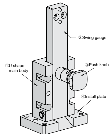
Aluminum U Shape Vertical Flip Component
