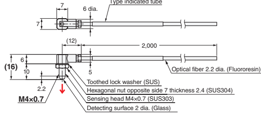
43-B E32-T12F 2M (Free Cutting)
