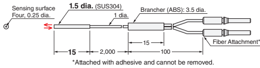
15-A E32-D22B 2M (No Cutting)
