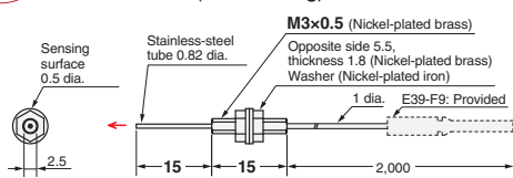
21-D E32-T21-S1 2M (Free Cutting)
