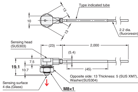
43-A2 E32-T11NFS 2M (Free Cutting)
