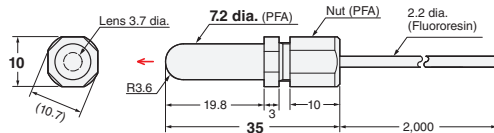
43-D E32-T14F 2M (Free Cutting)
