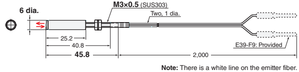
27-E E32-C31 2M (Free Cutting) + E39-F3B
