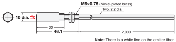
27-H E32-C91N 2M (Free Cutting) + E39-F18
