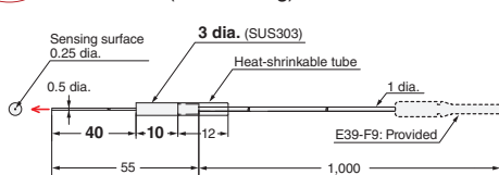
21-C E32-T33 1M (Free Cutting)
