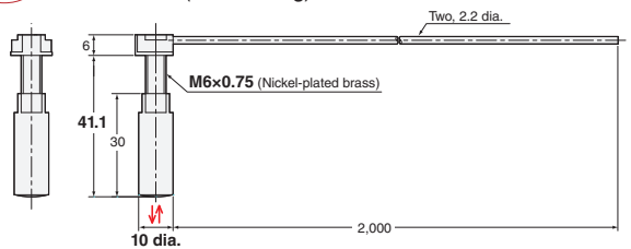
27-H E32-C91N 2M (Free Cutting) + E39-F18
